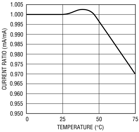
Normalized Fast Recharge Current vs Temperature
