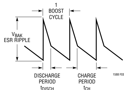
Figure 3. V_{BAK} Ripple
