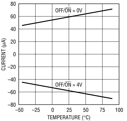
Gate Pin Current vs Temperature
