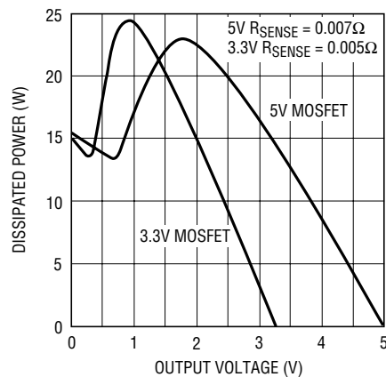
Figure 16. Worst-Case 5V and 3.3V MOSFET Dissipated Power vs Output Voltage
