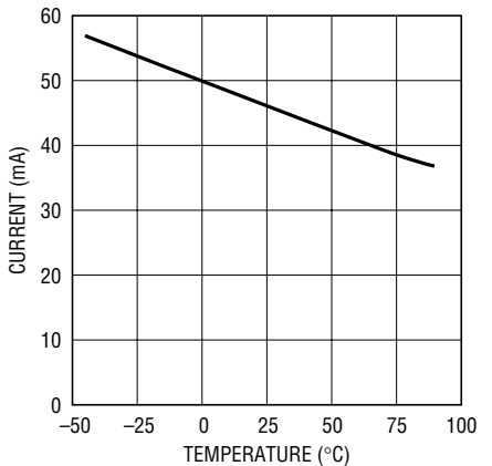
Timer Pin Off Current vs Temperature
