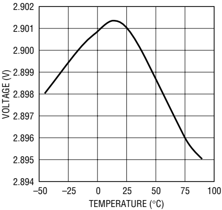
3.3V OUT Powergood Threshold Voltage vs Temperature
