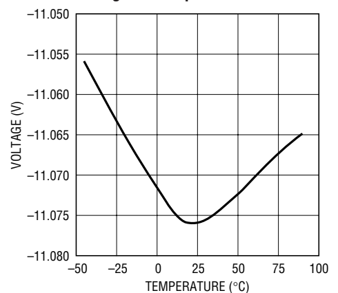
V EEIN Powergood Threshold Voltage vs Temperature
