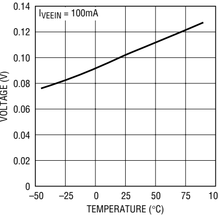
V EE Internal Switch Voltage Drop vs Temperature
