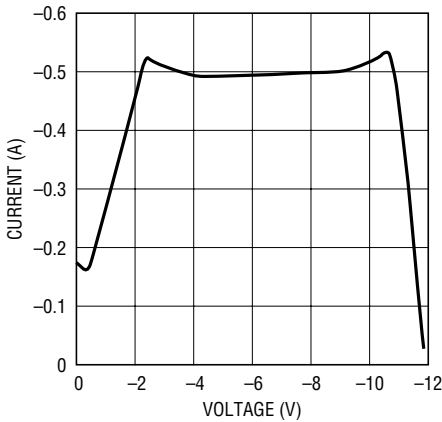
V EEOUT Current vs V EEOUT Voltage
