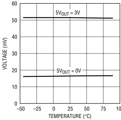
5V IN Foldback Current Limit Voltage vs Temperature
