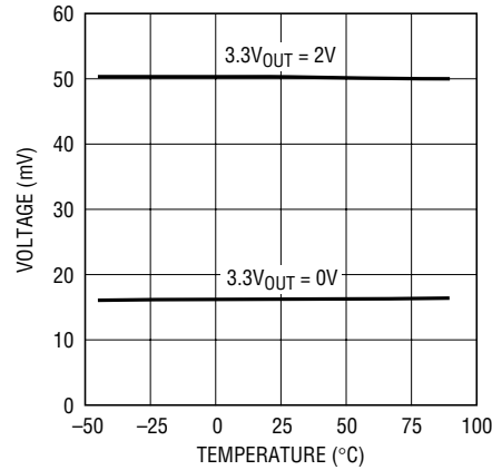
3.3V IN Foldback Current Limit Voltage vs Temperature
