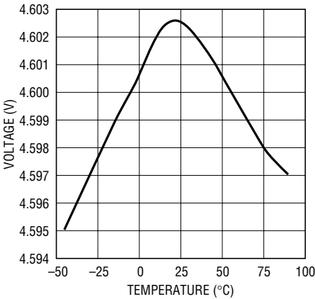
5V OUT Powergood Threshold Voltage vs Temperature
