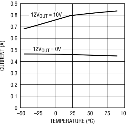
12V Foldback Current Limit vs Temperature
