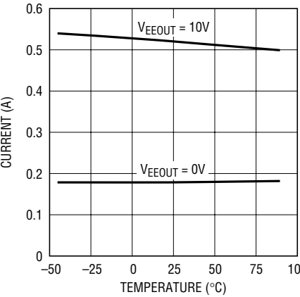
V EE Foldback Current Limit vs Temperature
