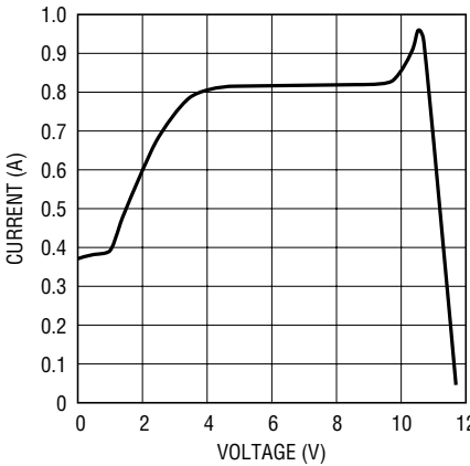
12V OUT Current vs 12V OUT Voltage
