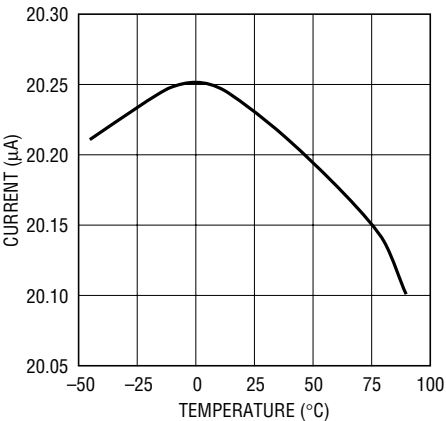
Timer Pin On Current vs Temperature
