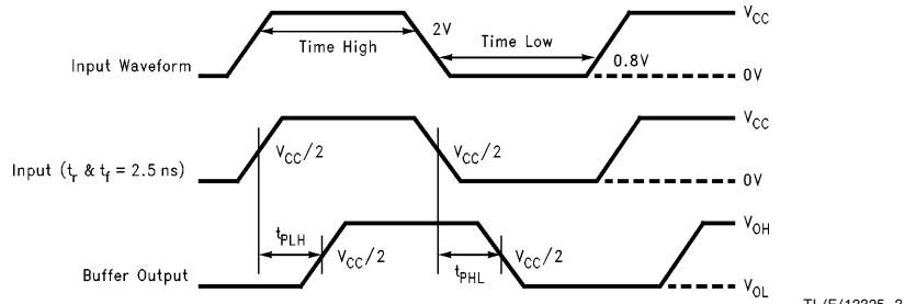
FIGURE 1. Buffer Waveforms
