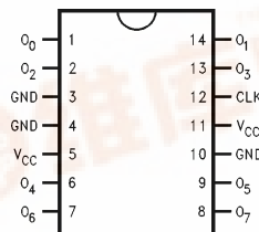
Pin Assignment for DIP and SOIC
