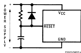
FIGURE 4. Recommended Reset Circuit
