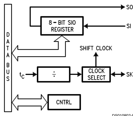
FIGURE 7. MICROWIRE/PLUS Block Diagram
