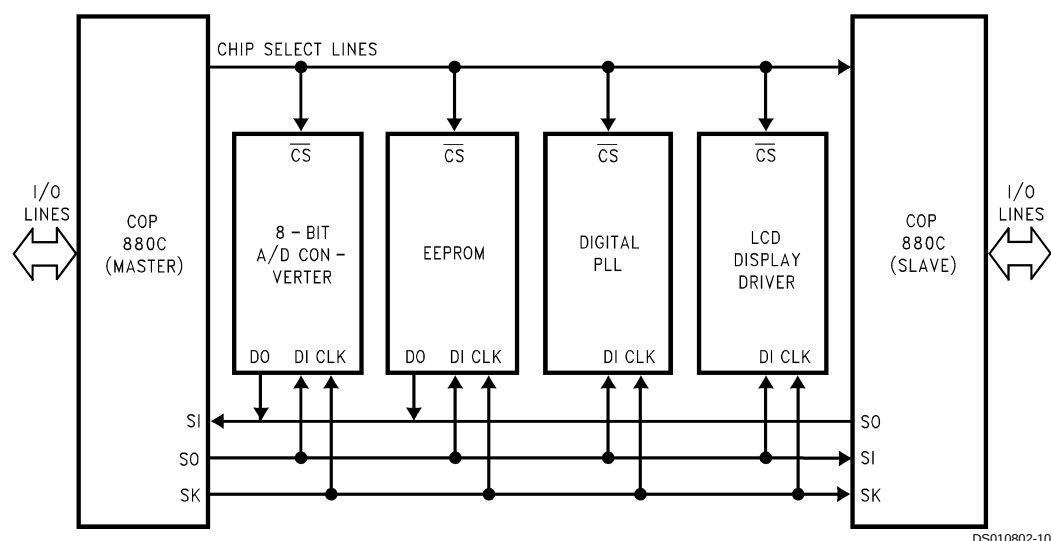
FIGURE 8. MICROWIRE/PLUS Application
