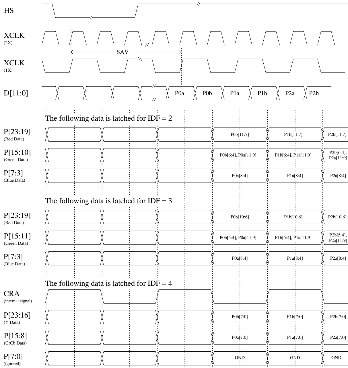
Figure 7: Multiplexed Input Data Formats (IDF = 2, 3, 4)
