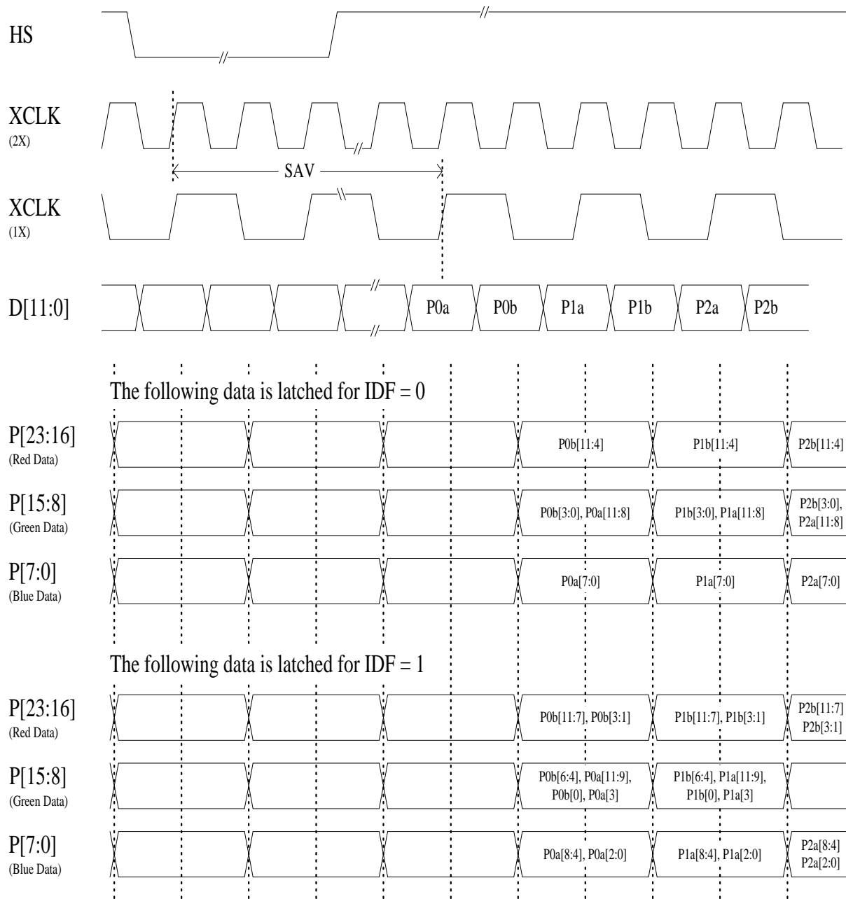
Figure 6: Multiplexed Input Data Formats (IDF = 0, 1)
