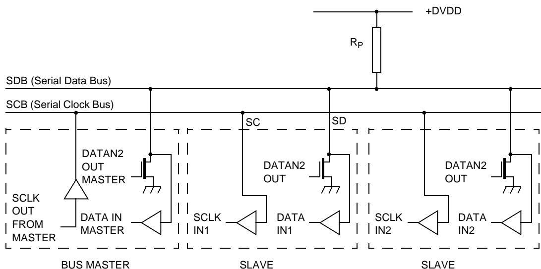
Figure 8: Connection of Devices to the Bus
