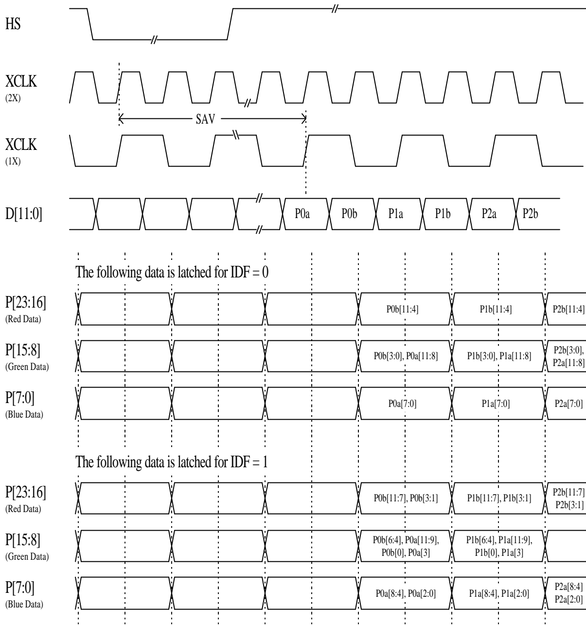
Figure 5: Multiplexed Input Data Formats (IDF = 0, 1)
