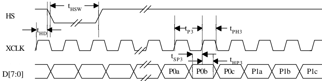
Figure 6: Multiplexed Pixel Data Transfer Mode (IDF = 6)
