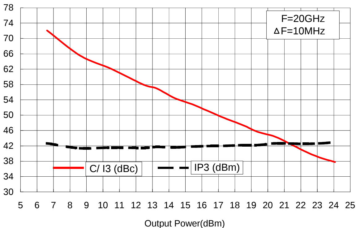
C/I3 &amp; IP3 versus total output power @ 20GHz
