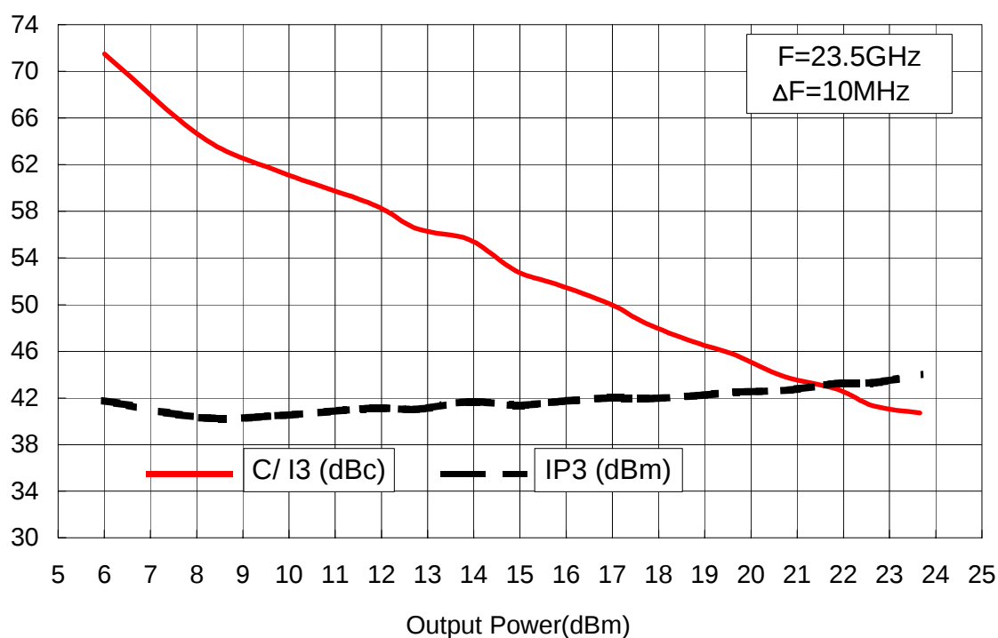
C/I3 &amp; IP3 versus total output power @ 23.5GHz
