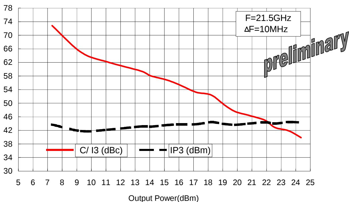
C/I3 &amp; IP3 versus total output power @ 21.5GHz
