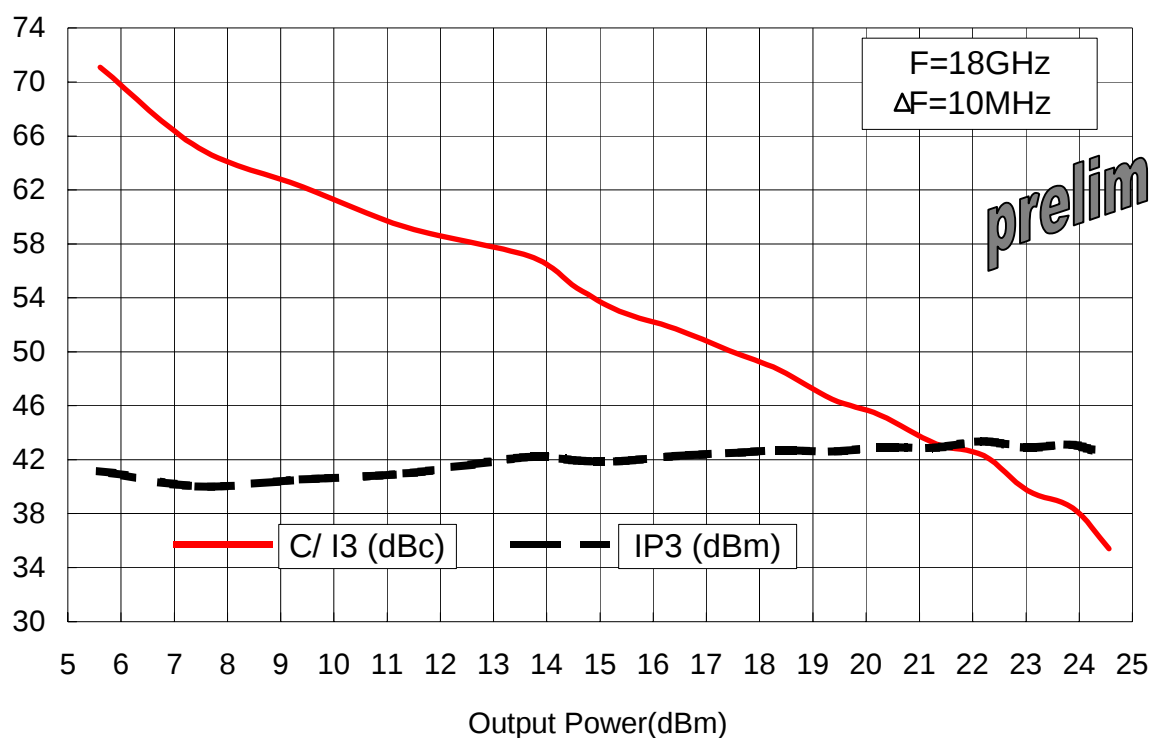
C/I3 &amp; IP3 versus total output power @ 18GHz
