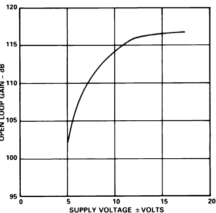
Figure 12. Open-Loop Gain vs. Supply Voltage
