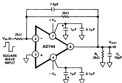
Figure 23a. Unity-Gain Inverter
