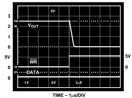
Figure 19. DAC Output Slew Rate Negative Transition
