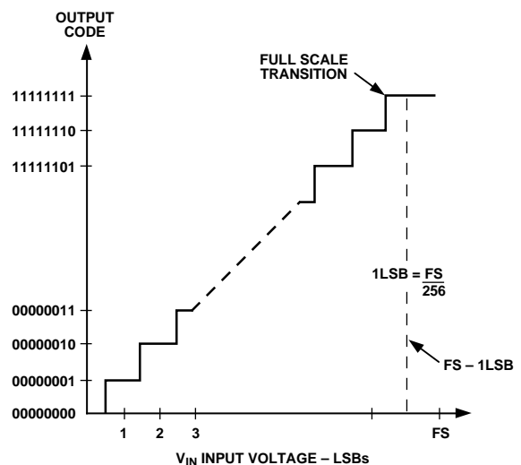
Figure 23. ADC 0 V to +3 V Input Transfer Characteristic
