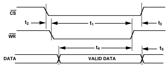
Figure 8. Write Cycle Timing
