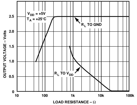
Figure 17. DAC Output Swing vs. Load Resistance
