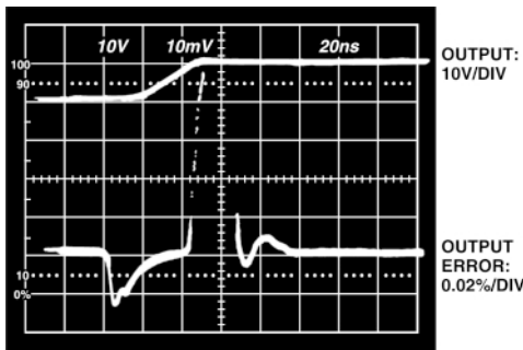
Figure 22. 0.01% Settling Time
