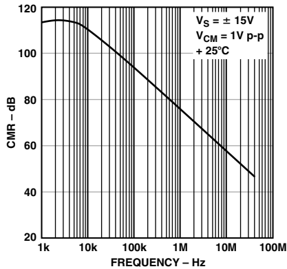
Figure 13. Common-Mode Rejection vs. Frequency
