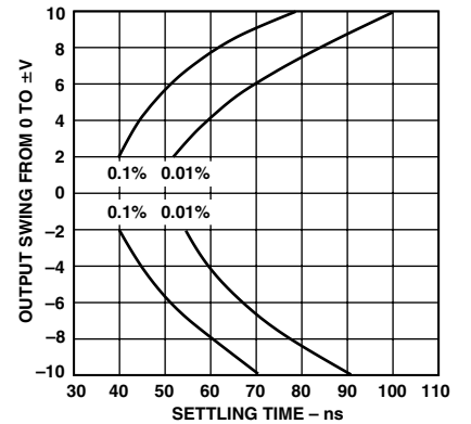
Figure 15. Output Swing and Error vs. Settling Time
