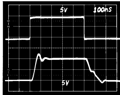
Figure 22b. Unity-Gain Follower Large Signal Pulse Response
