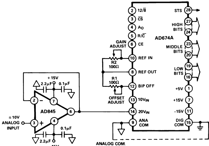
Figure 29. AD845 As ADC Unity Gain Buffer
