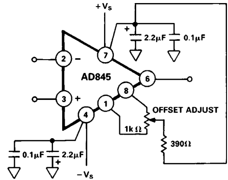
Figure 21. Offset Null Configuration Schematic
