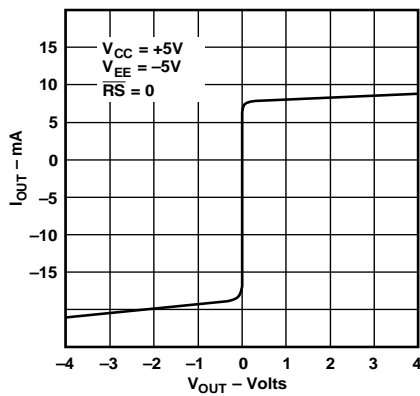
Figure 8. Output Current vs. Voltage
