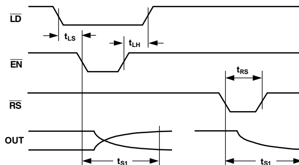
Figure 4. Write to DAC Register & Voltage Output Settling Timing ( \overline{\text{CS}} = High, Prevents Input Register Changes)
