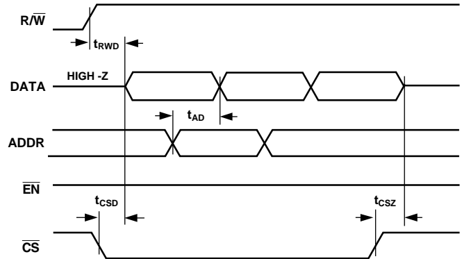
Figure 3. Readback Timing
