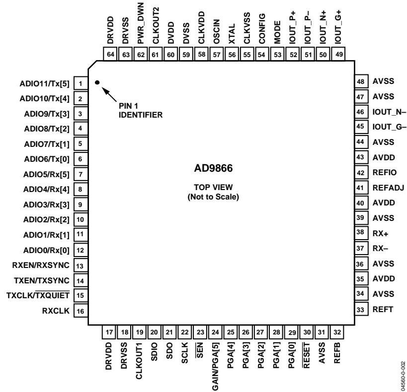
Figure 2. Pin Configuration
