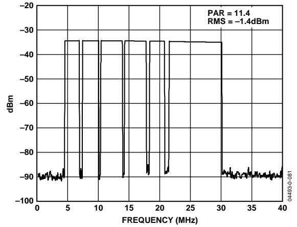
Figure 36. Spectral Plot of 111-Carrier OFDM Test Vector ( f_{DATA} = 80 MSPS, 2x Interpolation)
