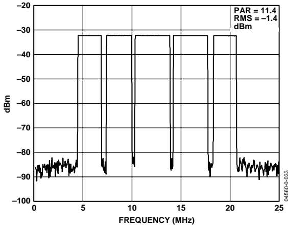
Figure 33. Spectral Plot of 84-Carrier OFDM Test Vector ( f_{DATA} = 50 MSPS, 4x Interpolation)
