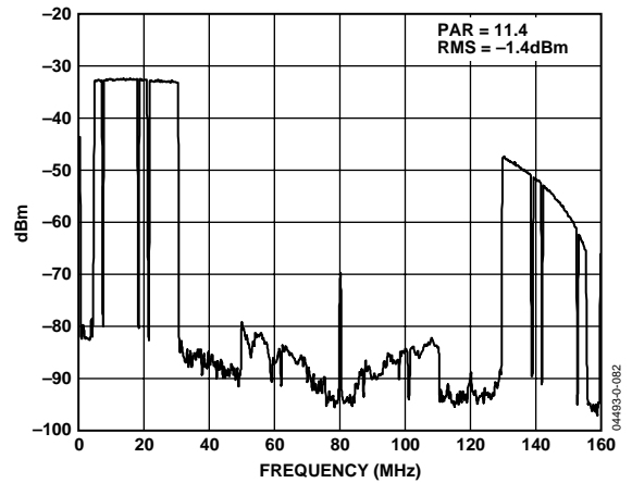
Figure 37. Wideband Spectral Plot of 111-Carrier OFDM Test Vector ( f_{DATA} = 80 MSPS, 2x Interpolation)
