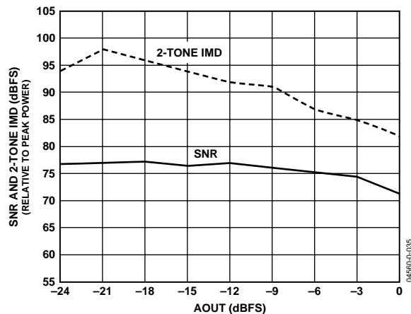
Figure 35. SNR and SFDR vs. P_{OUT} ( f_{OUT} = 12.55 MHz, f_{DATA} = 50 MSPS, 4x Interpolation)
