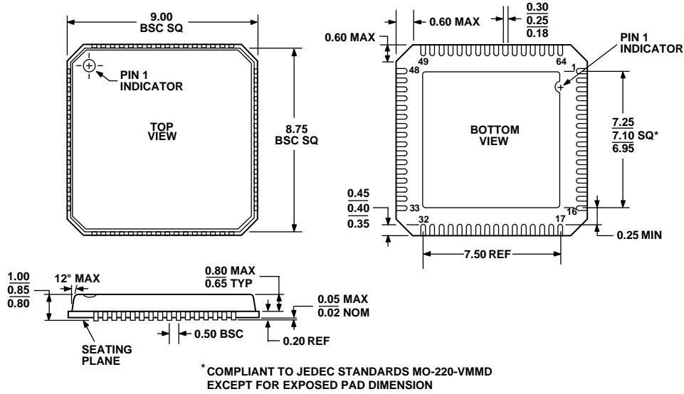
Figure 85. 64-Lead Lead Frame Chip Scale Package (LFCS) [CP-64-3] Dimensions shown in millimeters
