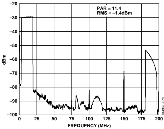
Figure 34. Wideband Spectral Plot of 88-Subcarrier OFDM Test Vector ( f_{DATA} = 50 MSPS, 4x Interpolation)
