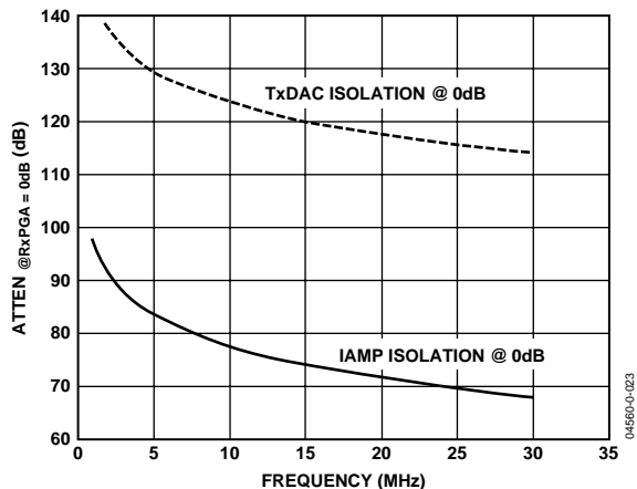
Figure 23. Rx to Tx Full-Duplex Isolation @ 0 RxPGA Setting (Note: ATTN_{@RxPGA=x\text{ dB}} = ATTN_{@RxPGA=0\text{ dB}} - RxPGA\text{ Gain} )
