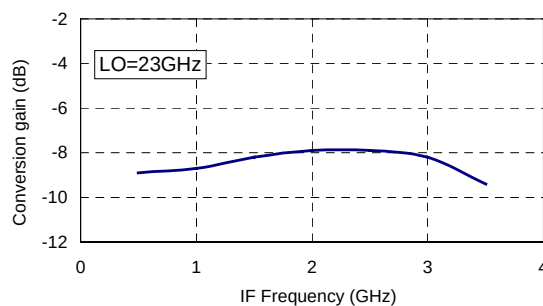
Conversion gain versus IF frequency LO Input power= 9dBm (1)
