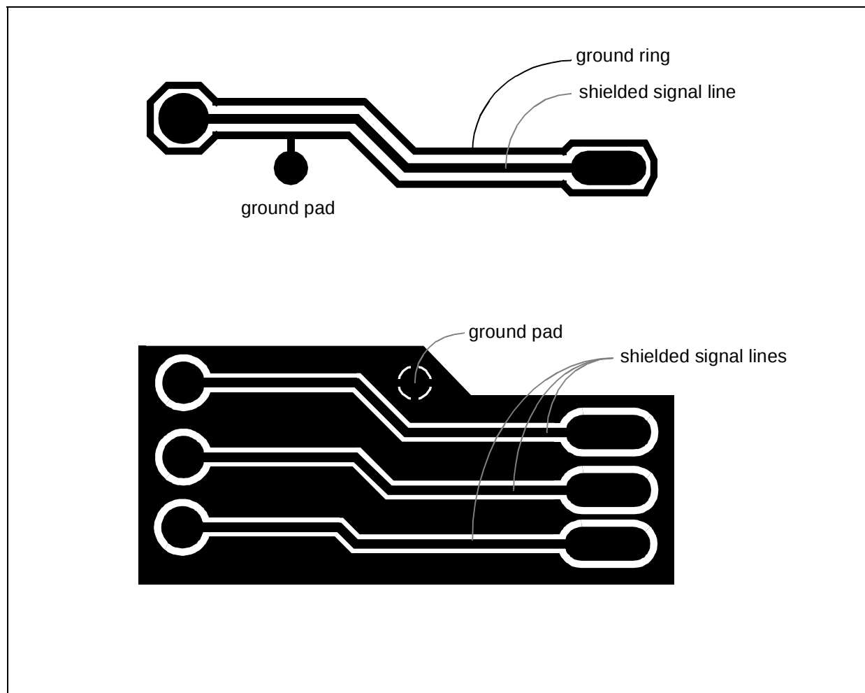
Figure 6-20. Shielding signals
