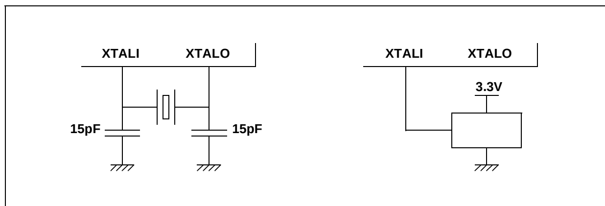
Figure 6-4. 14.31818 MHz stage
