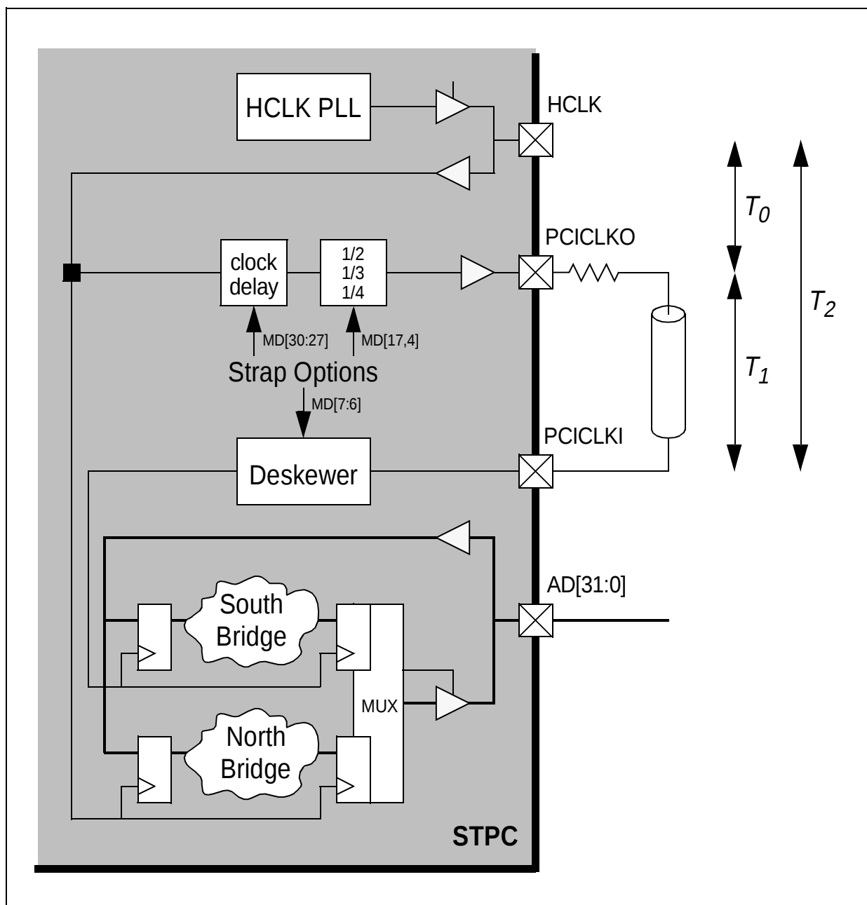
Figure 6-28. Clock Scheme
