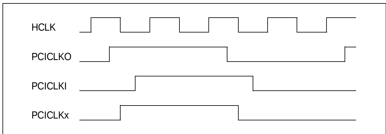
Figure 6-30. Clocks relationships
