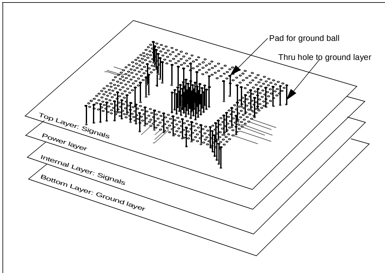
Figure 6-31. Ground Routing
