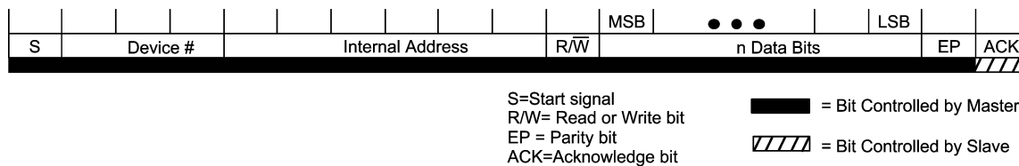
FIGURE 6. Write Transaction, master write data to LM41
