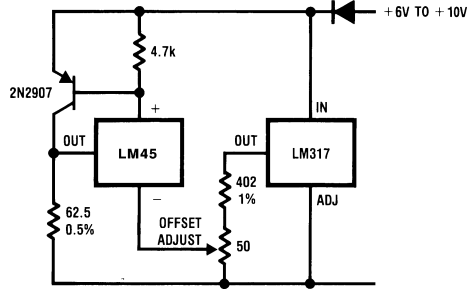
FIGURE 7. 4-to-20 mA Current Source ( 0^{\circ}\text{C} to +100^{\circ}\text{C} )
