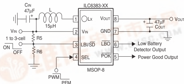
Figure 1. ILC6383CIR-XX
