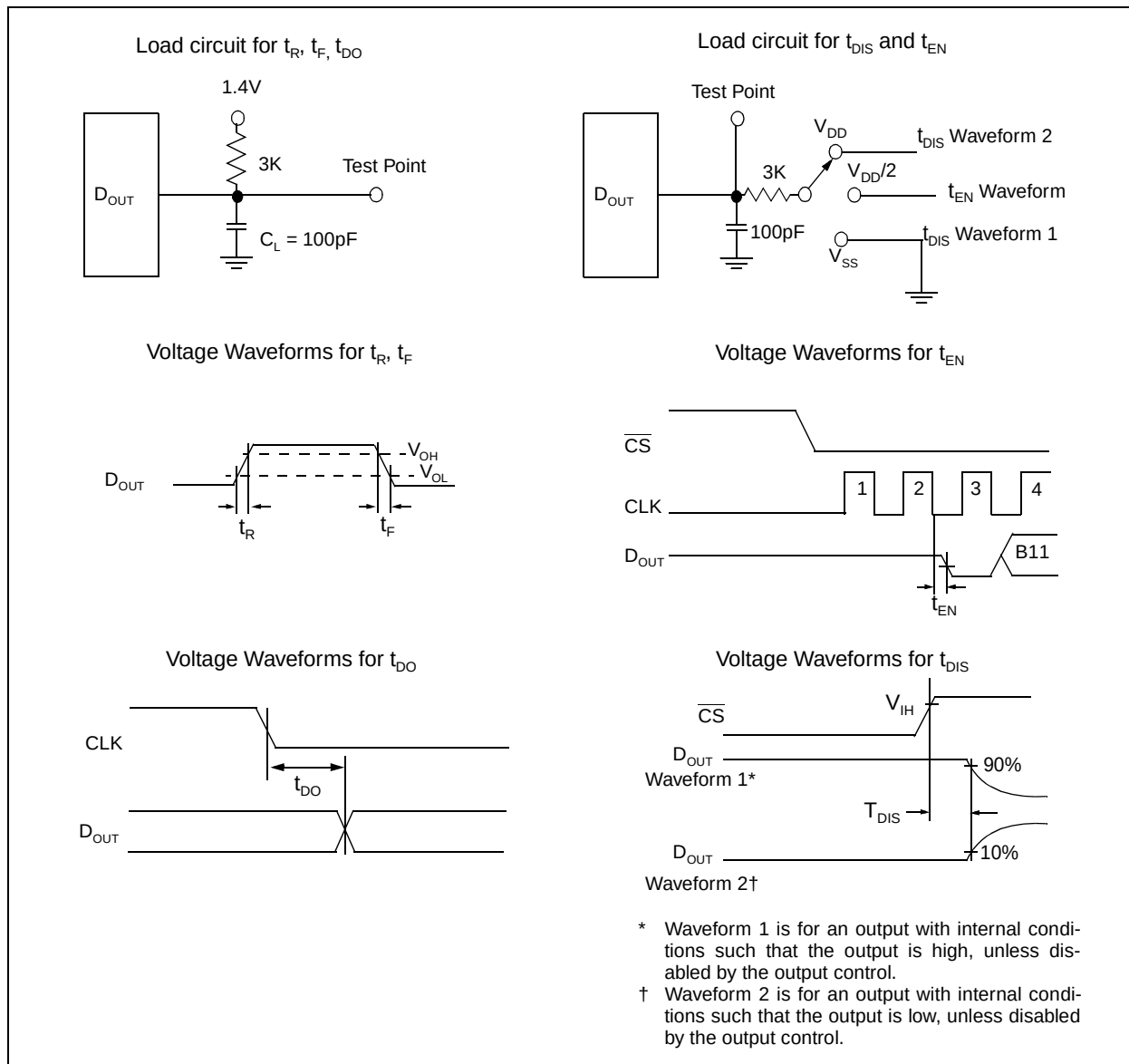
FIGURE 1-2: Test Circuits.
