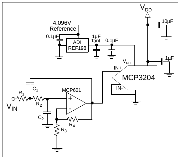
FIGURE 6-3: The MCP601 Operational Amplifier is used to implement a 2nd order anti-aliasing filter for the signal being converted by the MCP3204.
