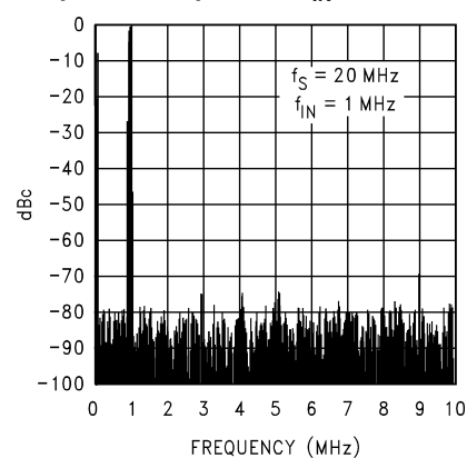
Spectral Response @ f_{IN} = 1\text{ MHz}
