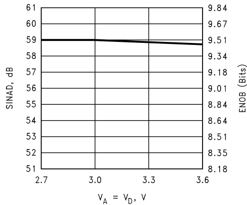
SINAD & ENOB vs. Supply Voltage @ f_{IN} = 1\text{ MHz to }9.5\text{ MHz}
