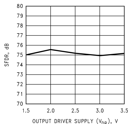
SFDR vs. V_{DR} @ f_{IN} = 4.7\text{ MHz}
