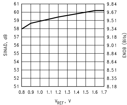
SINAD & ENOB vs. V_{REF} @ f_{IN} = 4.7\text{ MHz}
