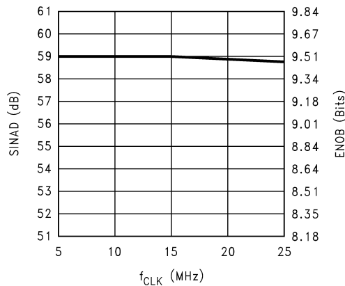
SINAD & ENOB vs. @ f_{CLK} ( f_{IN} = 9.5\text{ MHz} )
