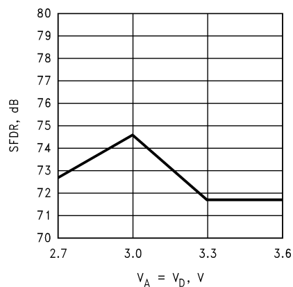
SFDR vs. Supply Voltage @ f_{IN} = 4.7\text{ MHz}
