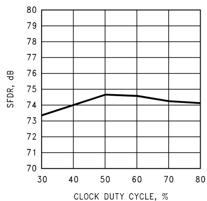
SFDR vs. Clock Duty Cycle @ f_{IN} = 4.7\text{ MHz}
