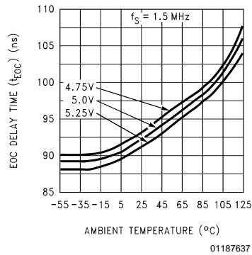
EOC Delay Time ( t_{EOC} ) vs Temperature
