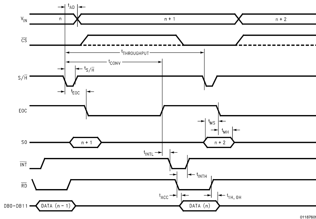
FIGURE 1. Interrupt Interface Timing (MODE = 0, OE = 1)
