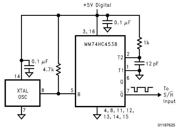
FIGURE 13. Crystal Clock Source
