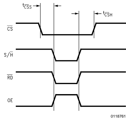
FIGURE 3. \overline{\text{CS}} Setup and Hold Timing for \text{S}/\overline{\text{H}} , \overline{\text{RD}} , and \text{OE}
