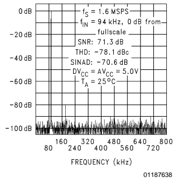
Spectral Response
