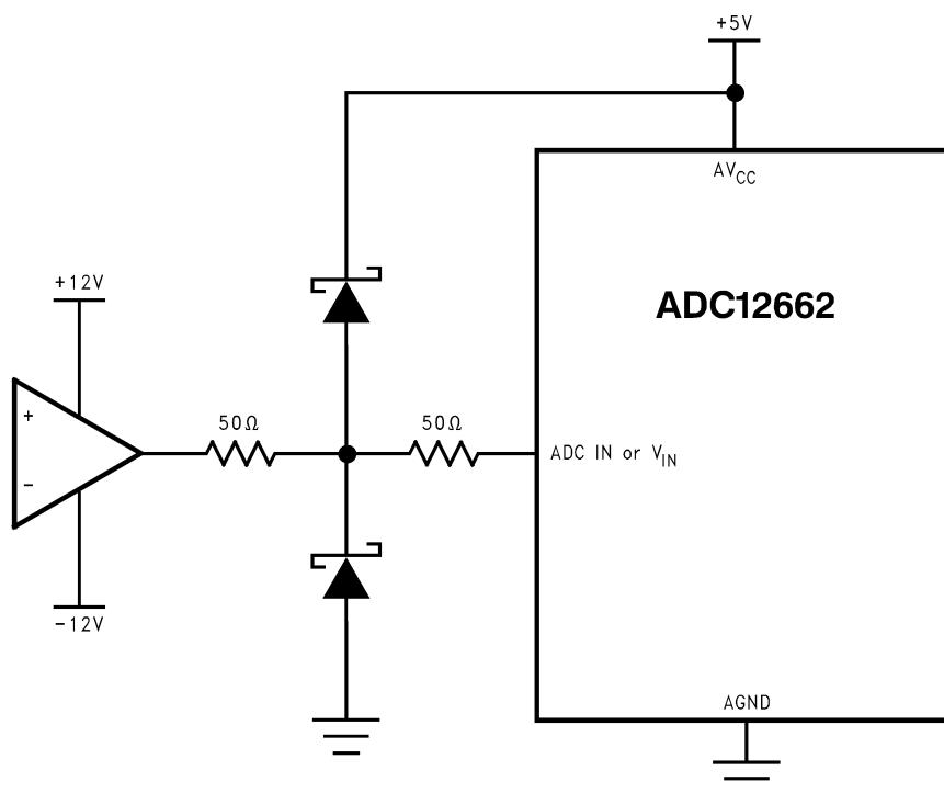
FIGURE 9. Input Protection
