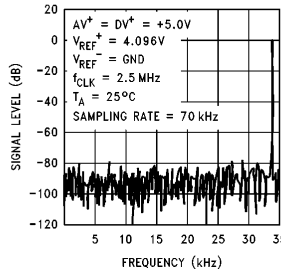
Spectral Response with 34 kHz Sine Wave
