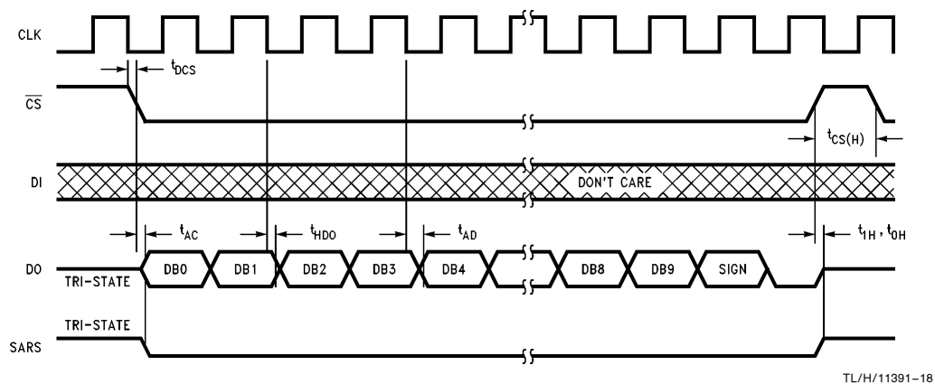
FIGURE 4. Delayed DO Timing
