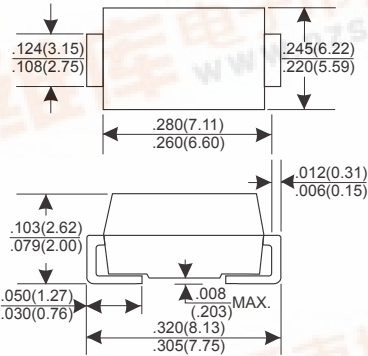
DO-214AB
