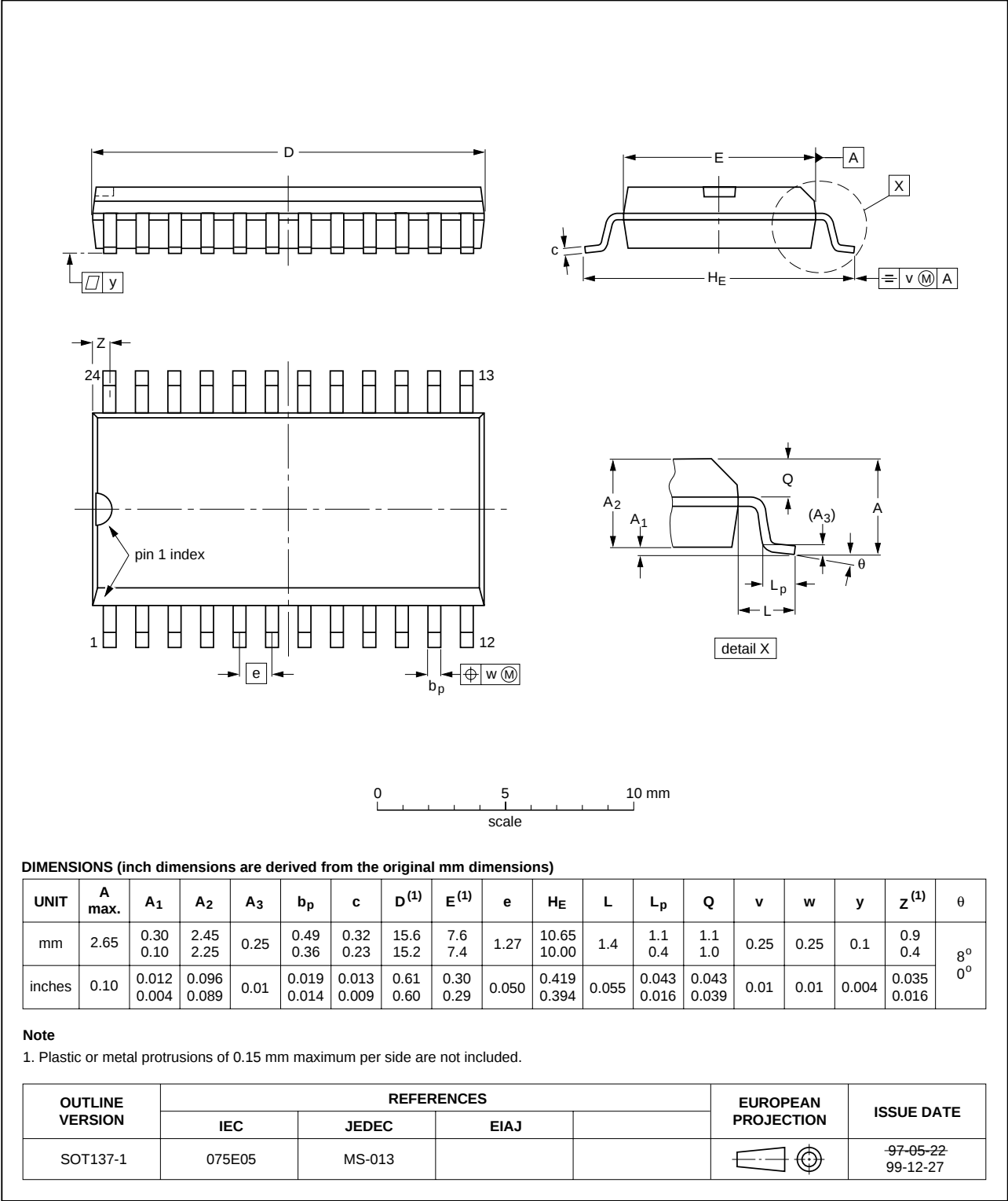
Fig 9. SO24 package outline (SOT137-1).
