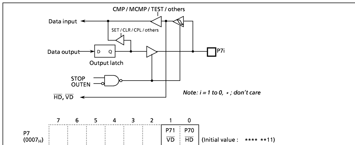
Figure 2-8. Ports P7
