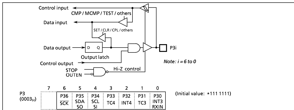
Figure 2-4. Port P3
