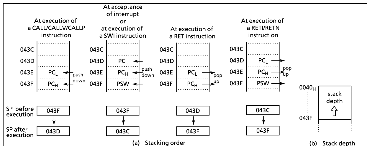
Figure 1-9. Stack
