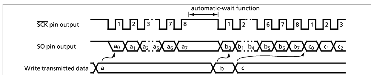
Figure 2-38. Automatic-wait Function
