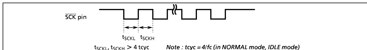
Figure 2-39. Maximum Data Transfer Frequency When External Clock Input
