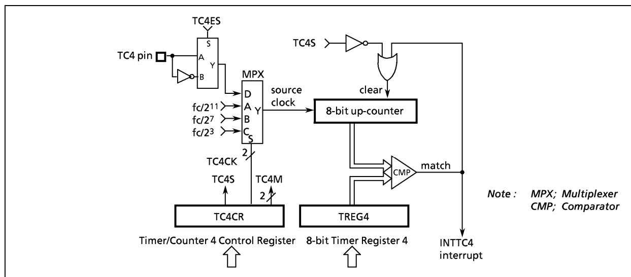
Figure 2-19. Timer/Counter 4
