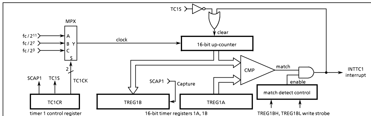
Figure 2-11. Timer 1 (TC1)
