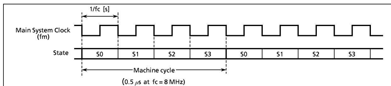
Figure 1-13. Machine Cycle
