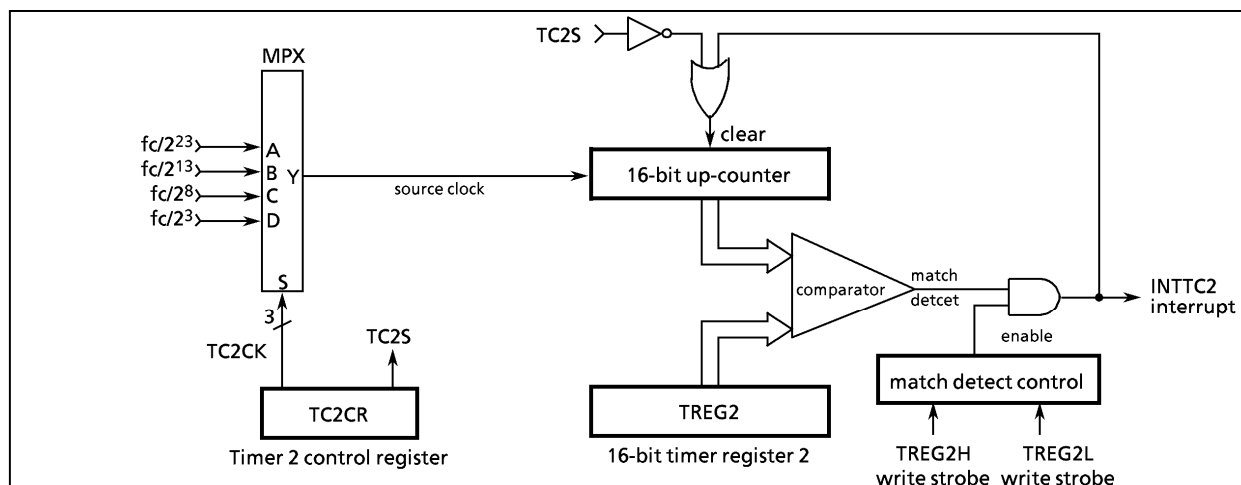
Figure 2-14. Timer 2 (TC2)
