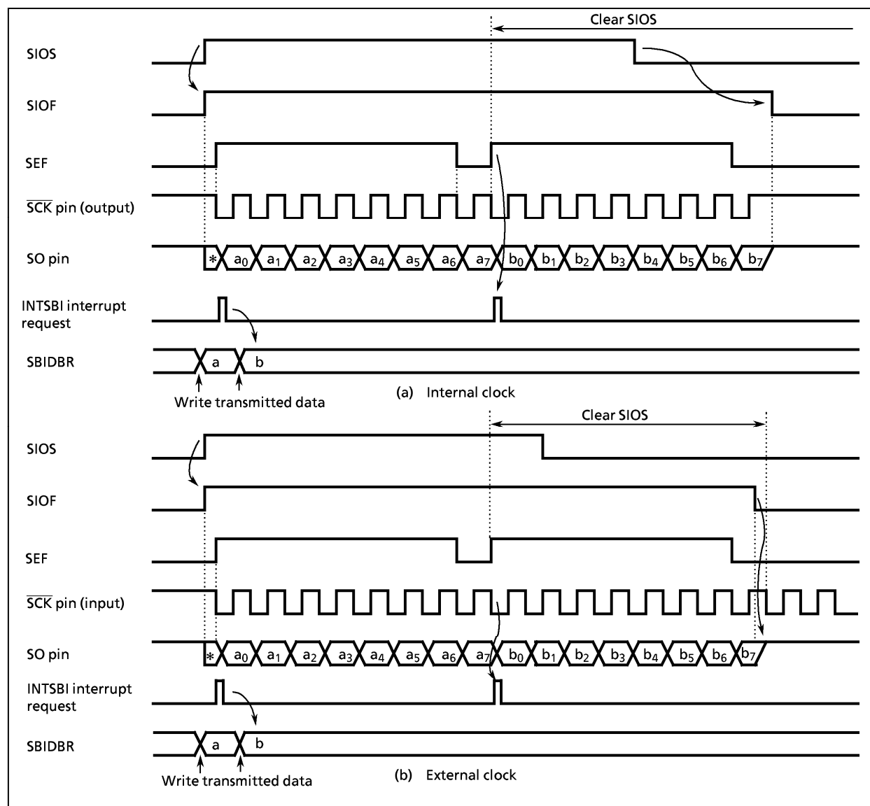
Figure 2-41. Transfer Mode
