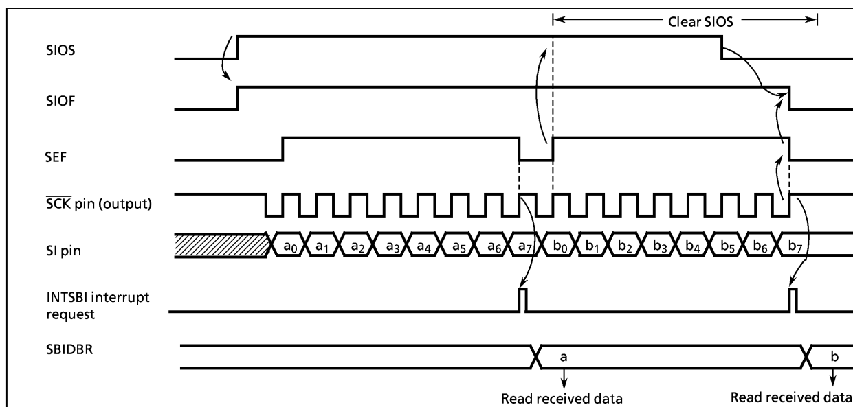
Figure 2-43. Receive Mode (Example : Internal clock)
