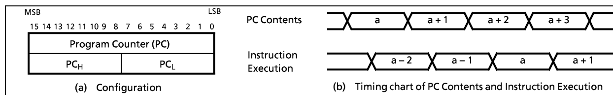
Figure 1-4. Program Counter
