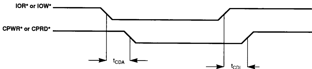
Figure 6–10. CPWR*/CPRD* Timing (ISA Bus)
