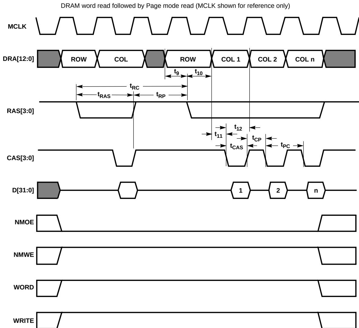
Figure 4-3. DRAM Read Cycles
