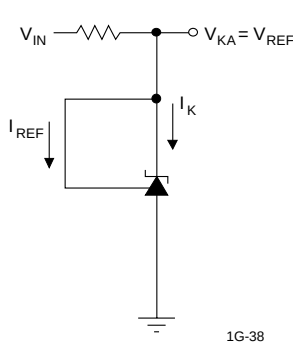
TEST CIRCUIT 1
