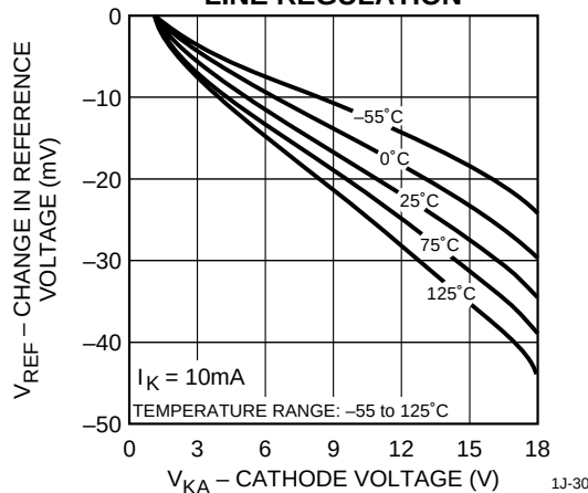
REFERENCE VOLTAGE LINE REGULATION
