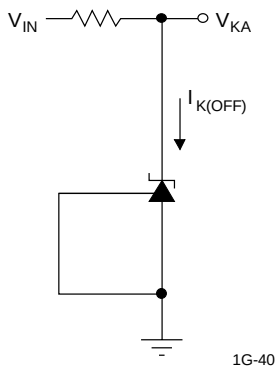
TEST CIRCUIT 3
