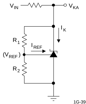
TEST CIRCUIT 2
