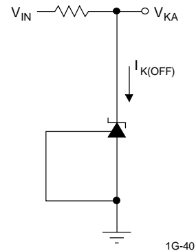
TEST CIRCUIT 3
