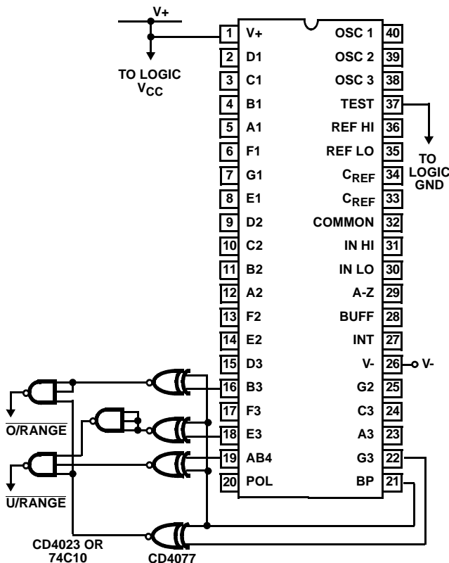
FIGURE 19. CIRCUIT FOR DEVELOPING UNDERANGE AND OVERANGE SIGNAL FROM ICL7106 OUTPUTS
