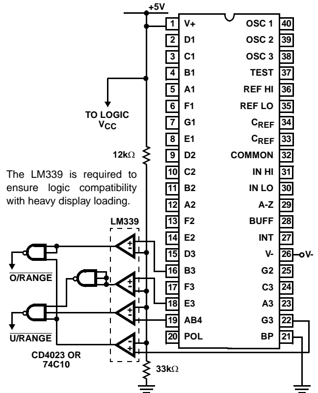
FIGURE 20. CIRCUIT FOR DEVELOPING UNDERANGE AND OVERANGE SIGNALS FROM ICL7107 OUTPUT
