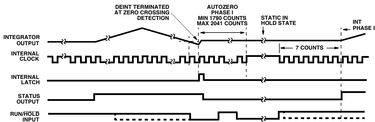
FIGURE 5. RUN/HOLD OPERATION
