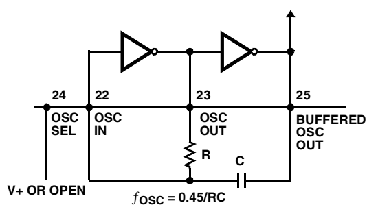
FIGURE 10. RC OSCILLATOR
