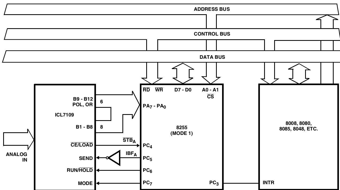
FIGURE 18. DIRECT ICL7109 - MC680X BUS INTERFACE
