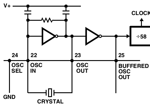
FIGURE 11. CRYSTAL OSCILLATOR
