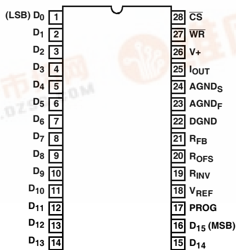
ICL7121 (OUTLINE DWG JI) TOP VIEW
