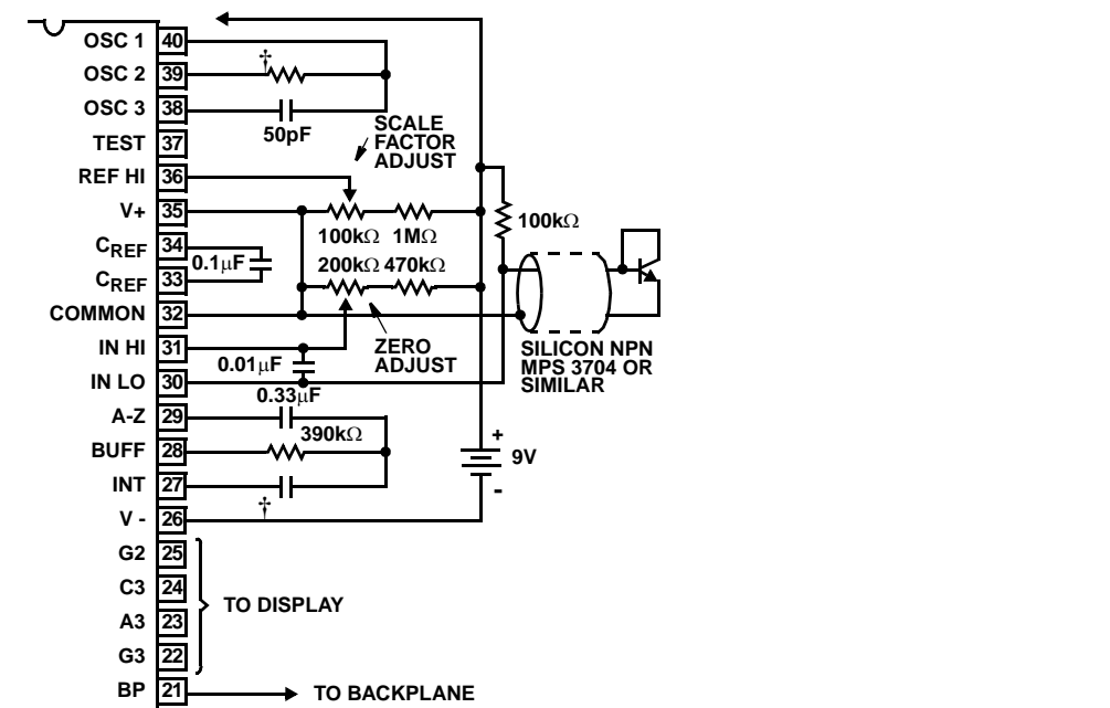
FIGURE 15. ICL7126 MEASURING RATIO METRIC VALUES OF QUAD LOAD CELL
