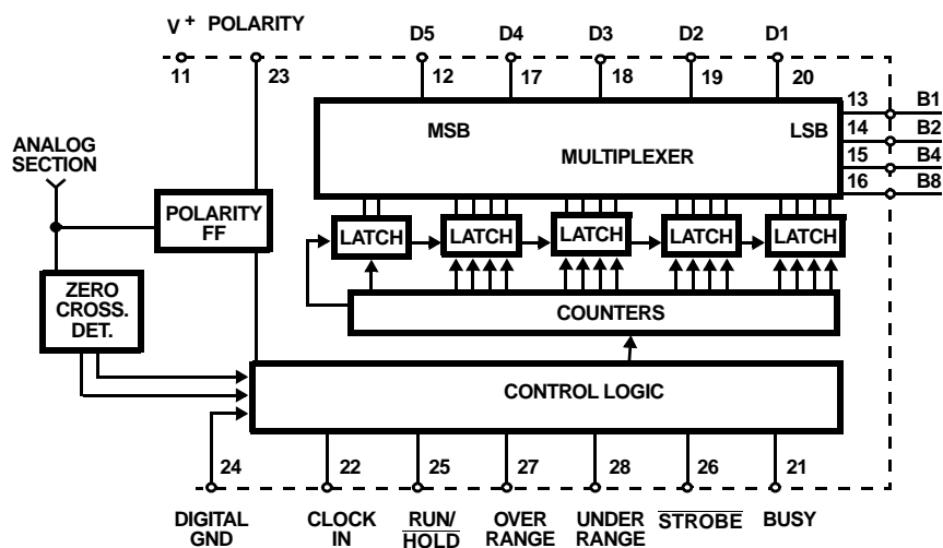
FIGURE 5. DIGITAL SECTION OF THE ICL7135
