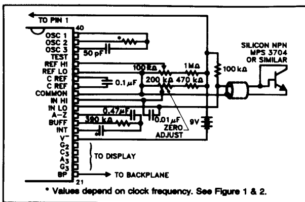
Figure 11. 7136 used as a Digital Centigrade Thermometer. A silicon diode-connected transistor has a temperature coefficient of about -2\text{mV}/^{\circ}\text{C} . Calibration is achieved by placing the sensing transistor in ice water and adjusting the zeroing potentiometer for a 000.0 reading. The sensor should then be placed in boiling water and the scale-factor potentiometer adjusted for a 100.0 reading.
