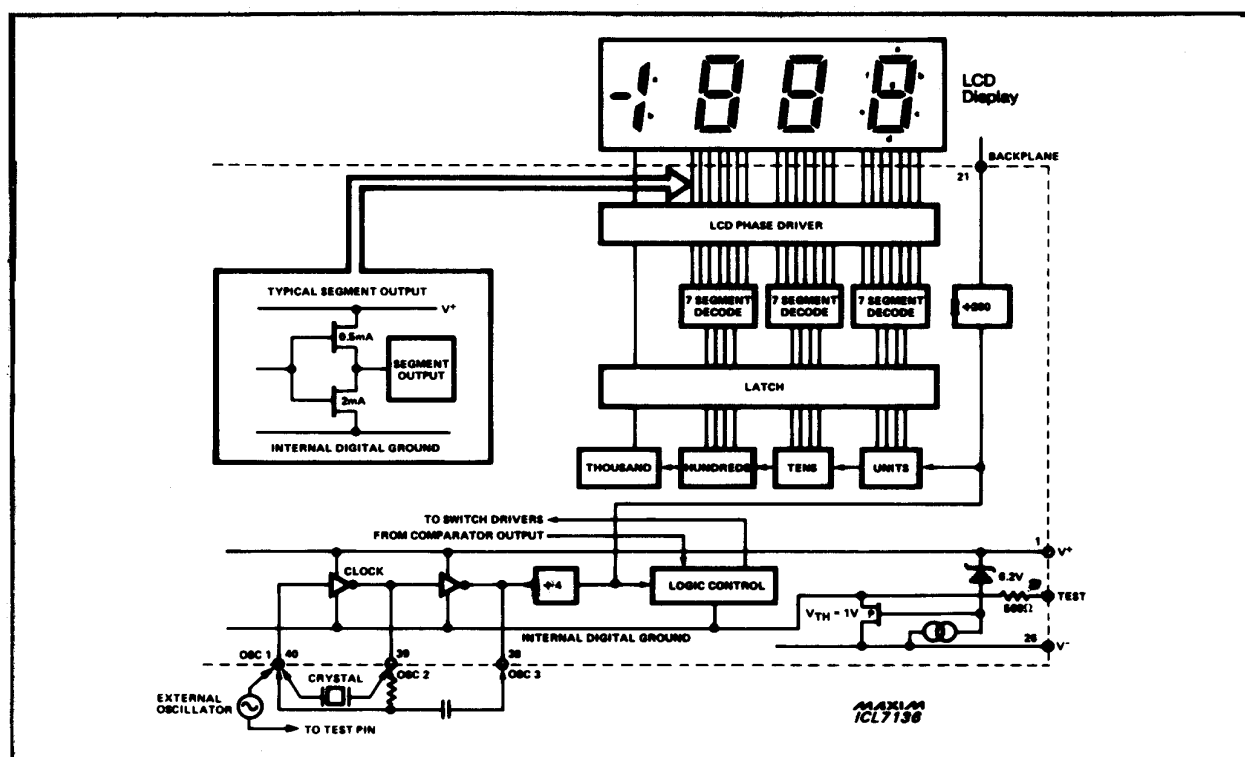
Figure 7. ICL7136 Digital Section
