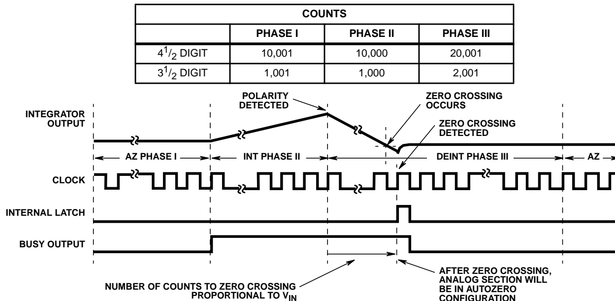
FIGURE 3. CONVERSION TIMING
