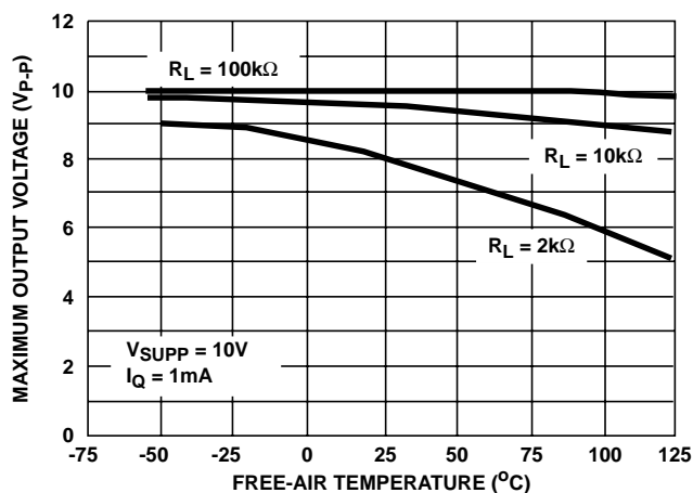
FIGURE 20. OUTPUT VOLTAGE vs FREE-AIR TEMPERATURE
