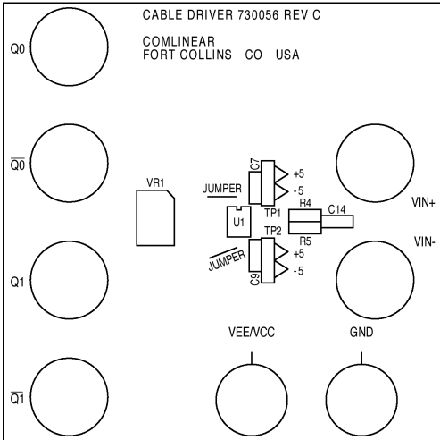
COMLINEAR LAYER1 SILK
