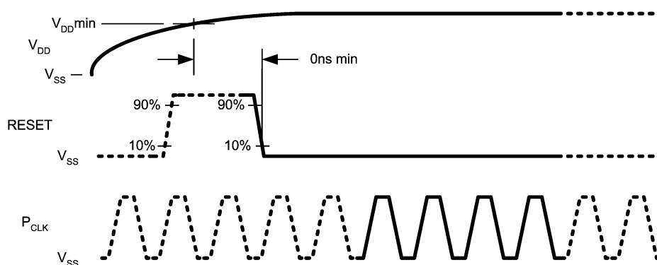
FIGURE 5. Power-On Reset Sequence with Manual Reset
