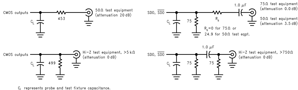
FIGURE 1. Test Loads
