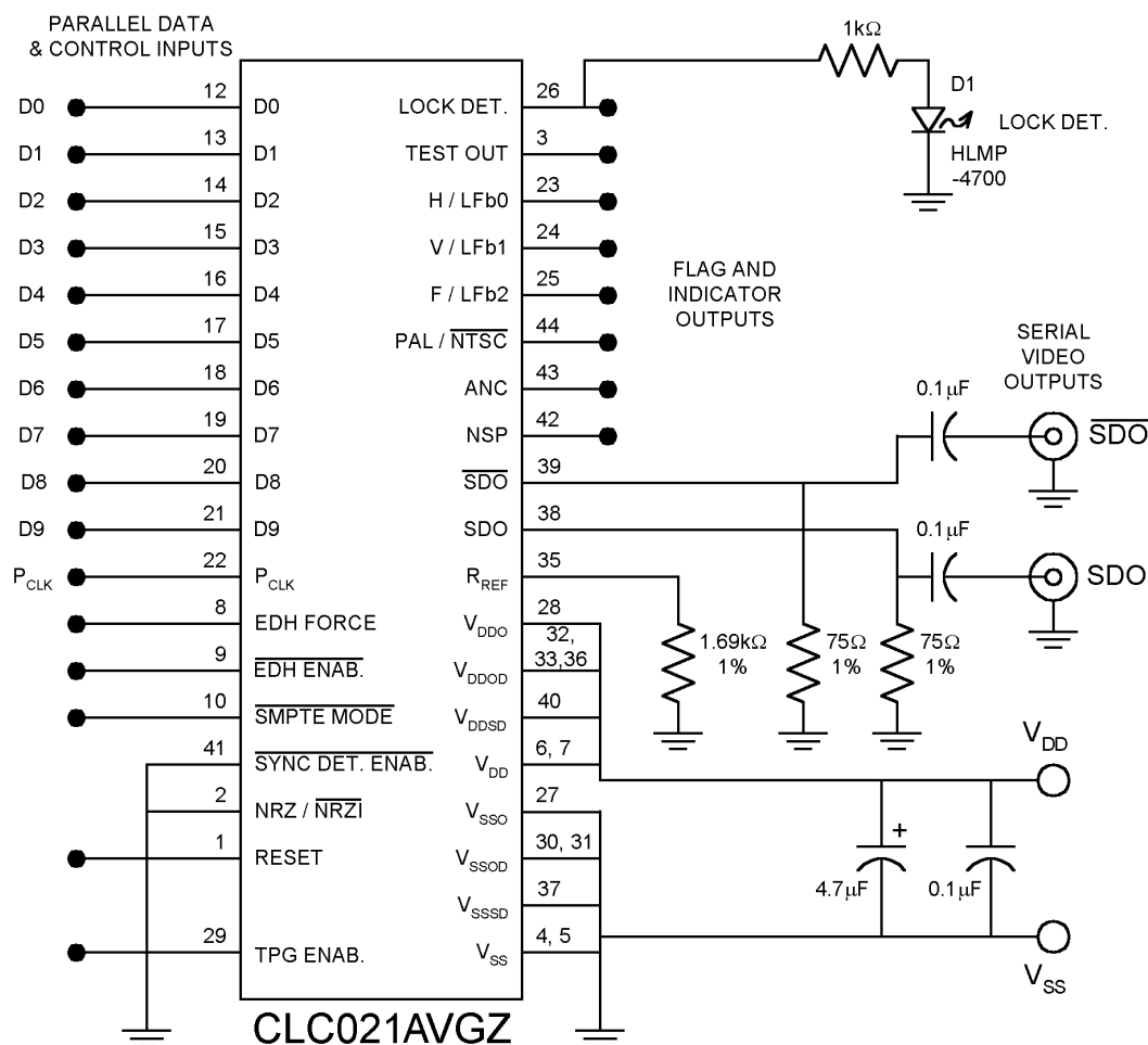
FIGURE 8. Typical Application Circuit
