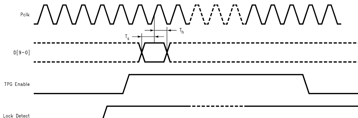
FIGURE 3. Setup and Hold Timing
