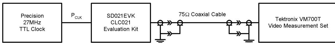
FIGURE 10. Jitter Test Circuit
