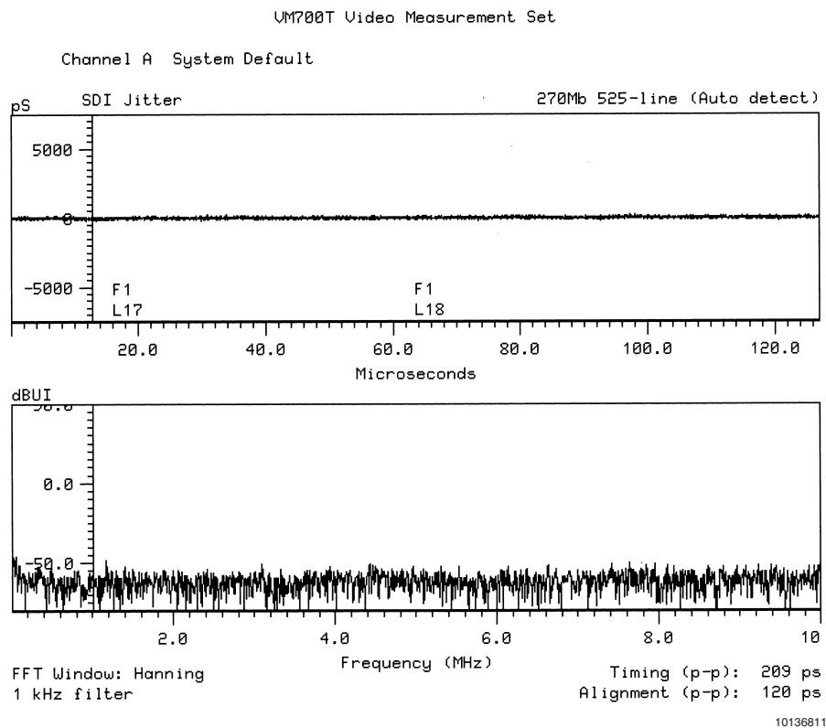
FIGURE 12. Jitter Plots
