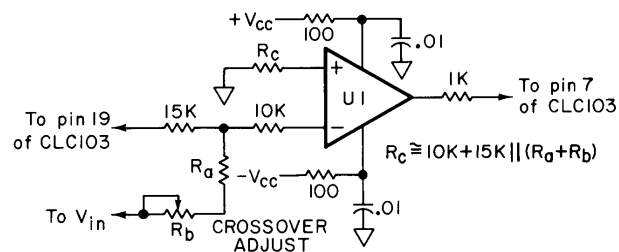
Figure 4: inverting gain composite amplifier
