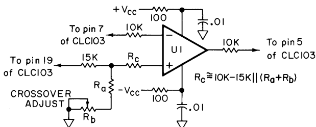
Figure 3: non-inverting gain composite amp
