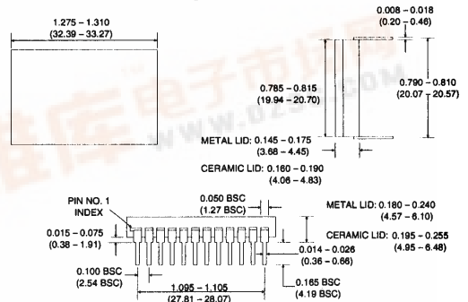
Package Dimensions
