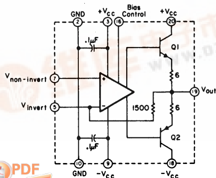
CLC103 Equivalent Circuit Diagram
