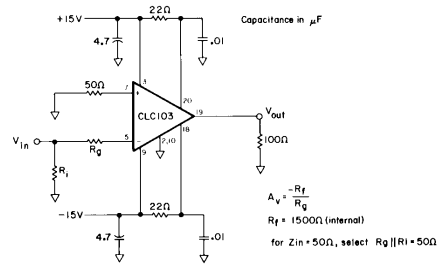
Figure 2: recommended inverting gain circuit
