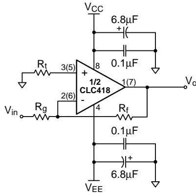
Figure 2: Inverting Gain
