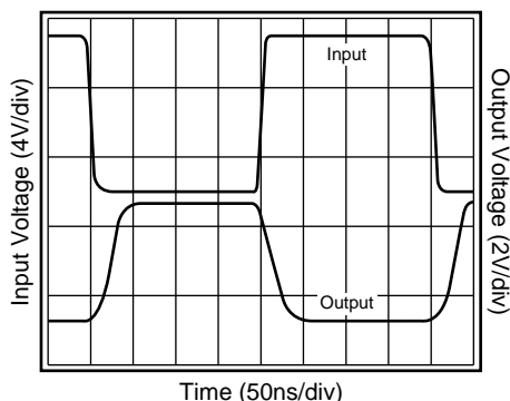
Figure 5: Overdrive Recovery
