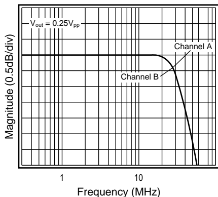
Figure 6: Channel Matching
