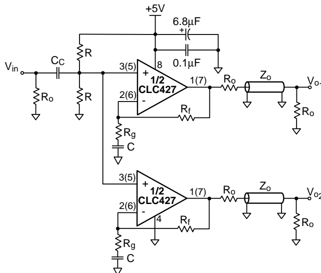
Figure 11: Distribution Amplifier
