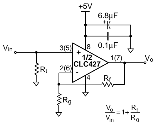
Figure 1: Non-inverting Configuration
