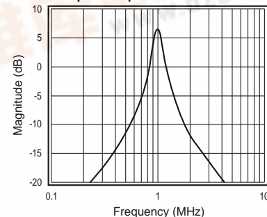
Bandpass Output
