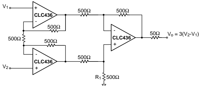
Figure 5: Instrumentation Amplifier
