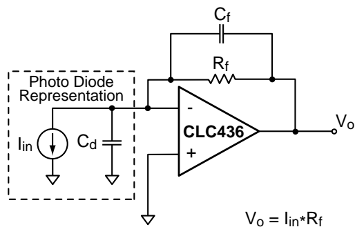
Figure 4: Transimpedance Amplifier
