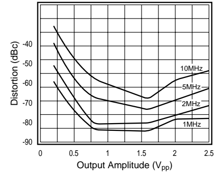
3rd Harmonic Distortion, R_L = 1k\Omega
