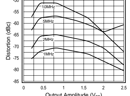
3rd Harmonic Distortion, R_L = 1k\Omega
