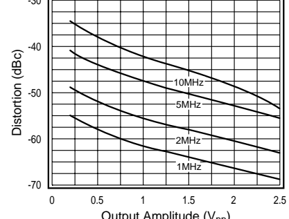
3rd Harmonic Distortion, R_L = 100\Omega
