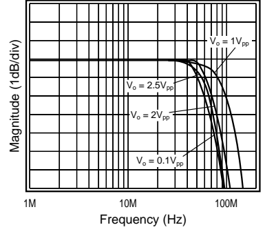
Gain Flatness
