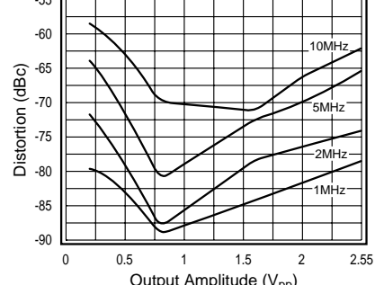
2nd Harmonic Distortion, R_L = 1k\Omega
