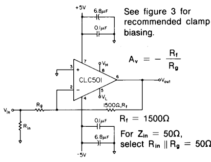
Figure 2: recommended inverting gain circuit
