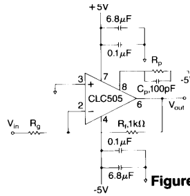
Figure 1: recommended non-inverting gain circuit
