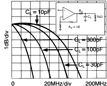
Recommended R_s vs Load Capacitance
