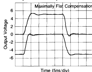
Settling Time into a 50pF Load
