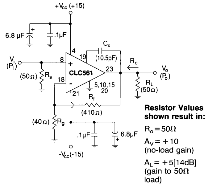
Figure 1: Test Circuit
